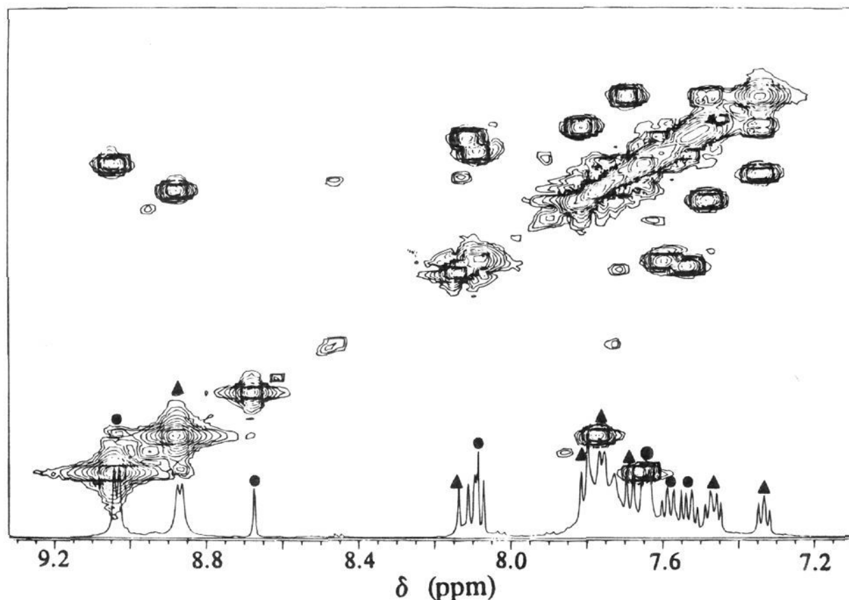
Figure 10. Partial 2D COSY spectrum recorded for 5 in acetone- d_6 at -30 °C: marked are the two sets of matching resonances with the upfield protons marked ( \blacktriangle ) and the corresponding downfield shifted protons marked ( \bullet ). Signals occurring at 9.04, 8.86, 7.79, 7.75, 7.73, and 7.64 ppm are attributed to the cyclophane and all other signals are due to the anthracene subunits.
