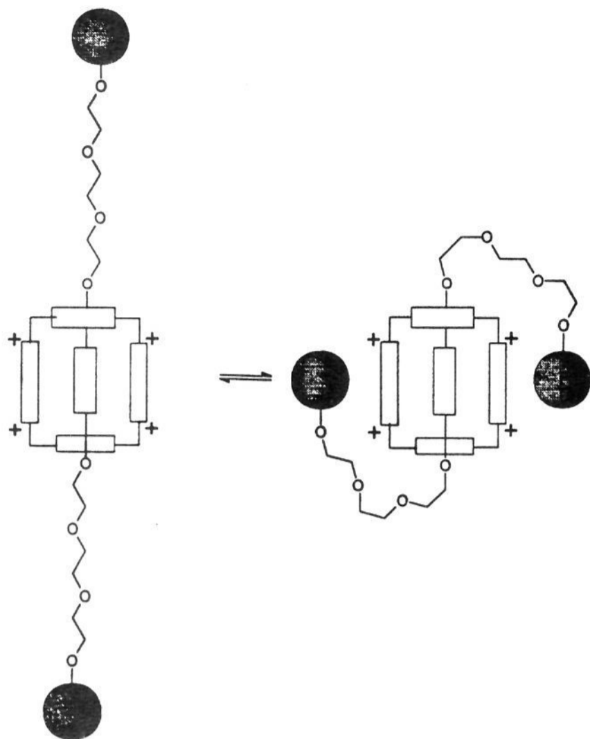
Figure 5. Major conformational exchange process for the one-station [2]rotaxanes. The cyclophane can oscillate along the extended string in the "open" conformer while the terminal stoppers associate with the exterior of the cyclophane in the "closed" conformer.
