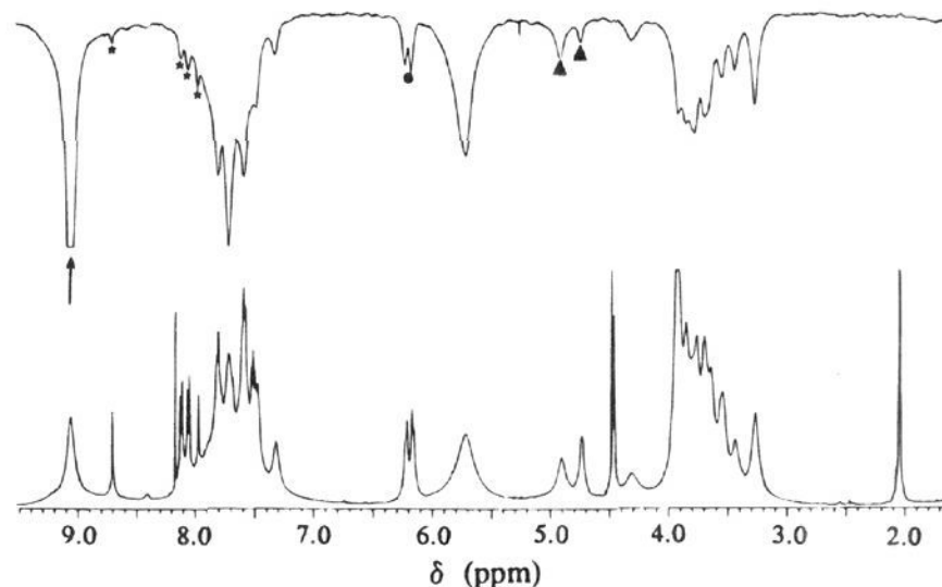
Figure 12. NOE difference spectrum recorded for 5 in acetone- d_6 at -80 °C under irradiation ( \delta = 9.05 ppm) into the CH( \alpha ) protons on the cyclophane. The resonances marked (*) refer to protons on the anthracene subunit, ( \bullet ) refers to protons on the unoccupied station, and ( \blacktriangle ) refers to protons adjacent to the ester group.
