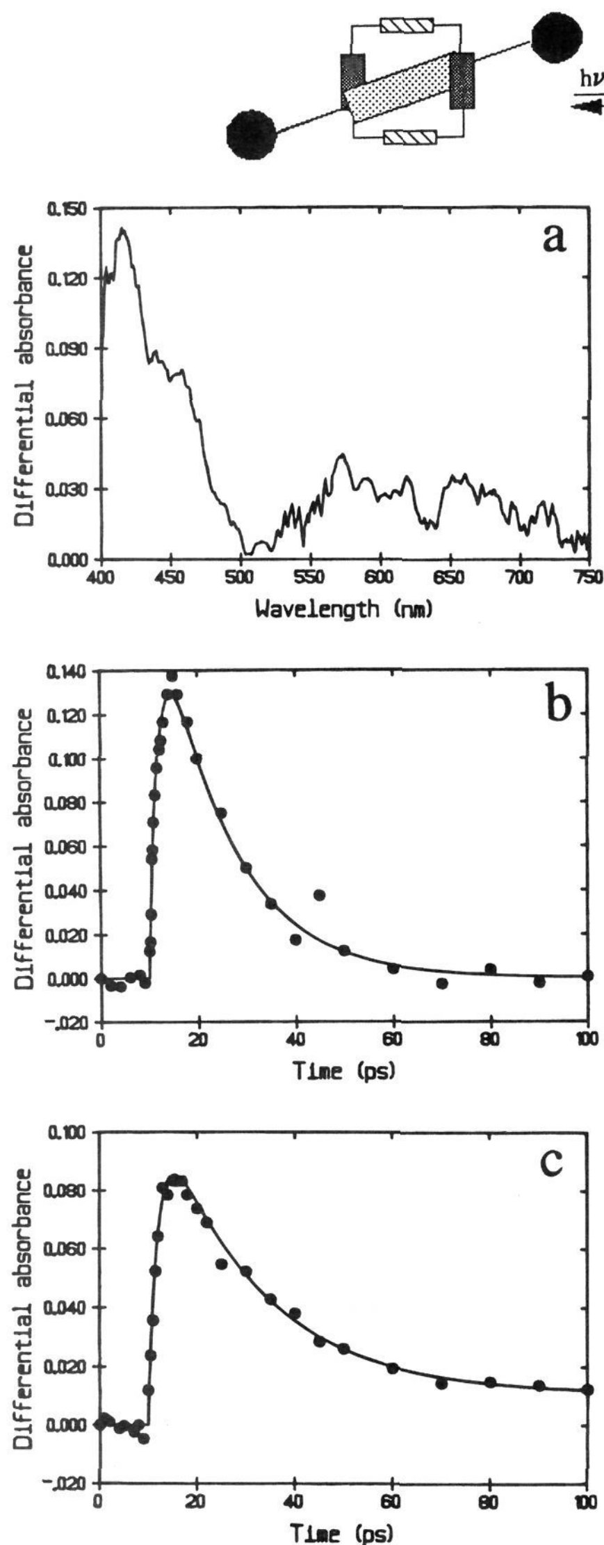
Figure 15. (a) Transient differential absorption spectrum recorded 2 ps after excitation of 1 in \text{CH}_3\text{CN} with a sub-ps laser pulse at 440 nm. (b) Kinetic profile recorded at 400 nm for the above experiment. (c) Kinetic profile recorded at 400 nm for 2 after irradiation under identical conditions.
