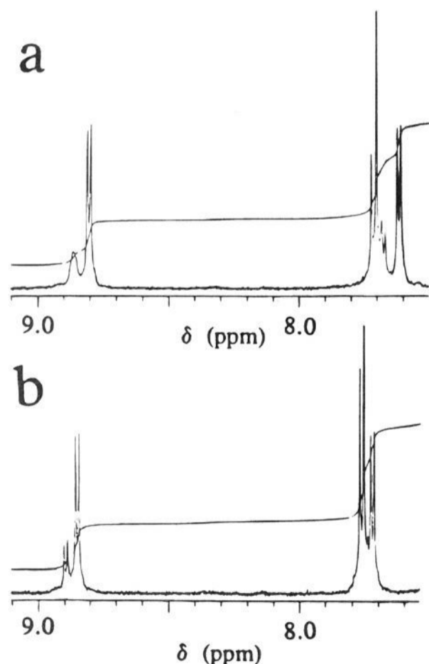
Figure 6. Partial ^1\text{H} NMR (500 MHz) spectra recorded for 3 in \text{CD}_3\text{CN} at (a) -35\text{ }^\circ\text{C} and (b) +25\text{ }^\circ\text{C} showing the aromatic region.
